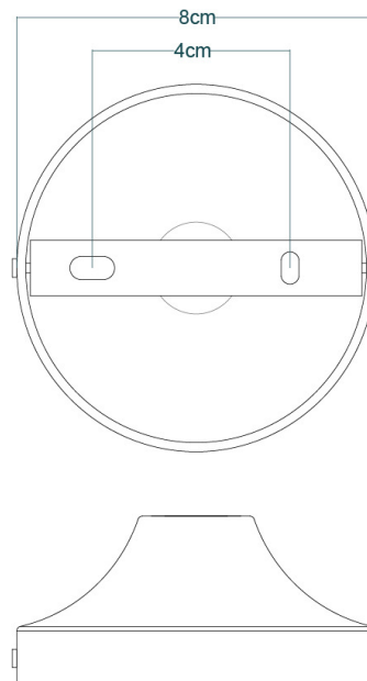
Fixing Bracket MLWB03 | Natural Brass
